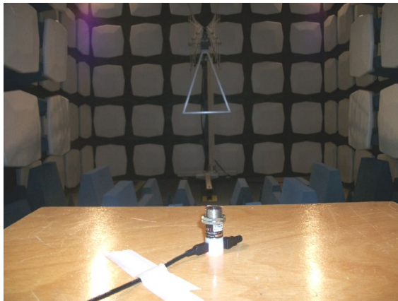
Photos 14 and 15 - Radiated Disturbance Immunity
