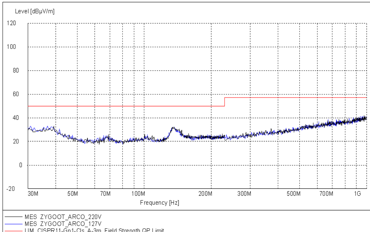
Graph 2 Radiated Emission Preliminary Test Results – Default Configuration – Power Supply 127V @ 60 Hz / 220V @ 60 Hz – Sample 5284
