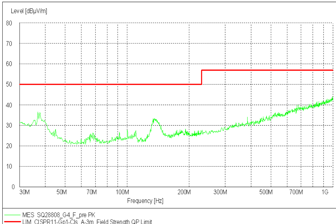
Graph 1 Radiated Emission Test Results – Default Configuration – Power Supply 220V @ 60 Hz (24 Vdc output) – Sample 5284
