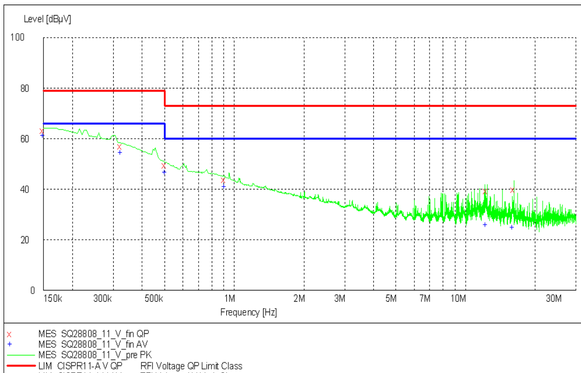
Graph 3 Conducted Emission in Electric Power Terminals Test Results – Default Configuration – Power Supply 24Vdc – Sample 5252
