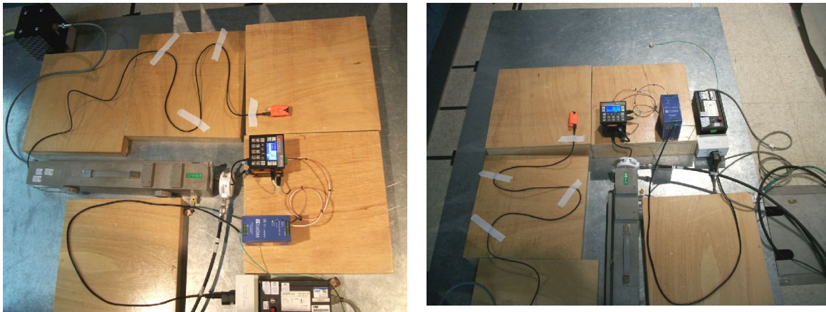
Photos 15 and 16 - Immunity to Conducted RF
