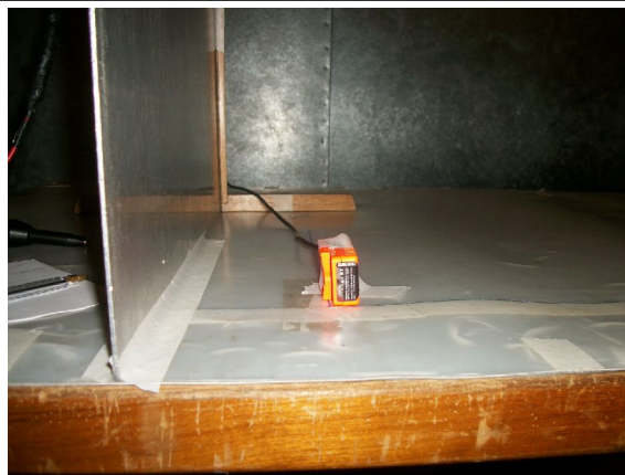
Photo 22 Horizontal left view and vertical rear view of EUT
