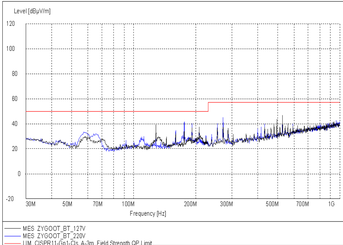
Graph 2 Radiated Emission Preliminary Test Results – Default Configuration – Power Supply 127V @ 60 Hz / 220V @ 60 Hz – Sample 5252
