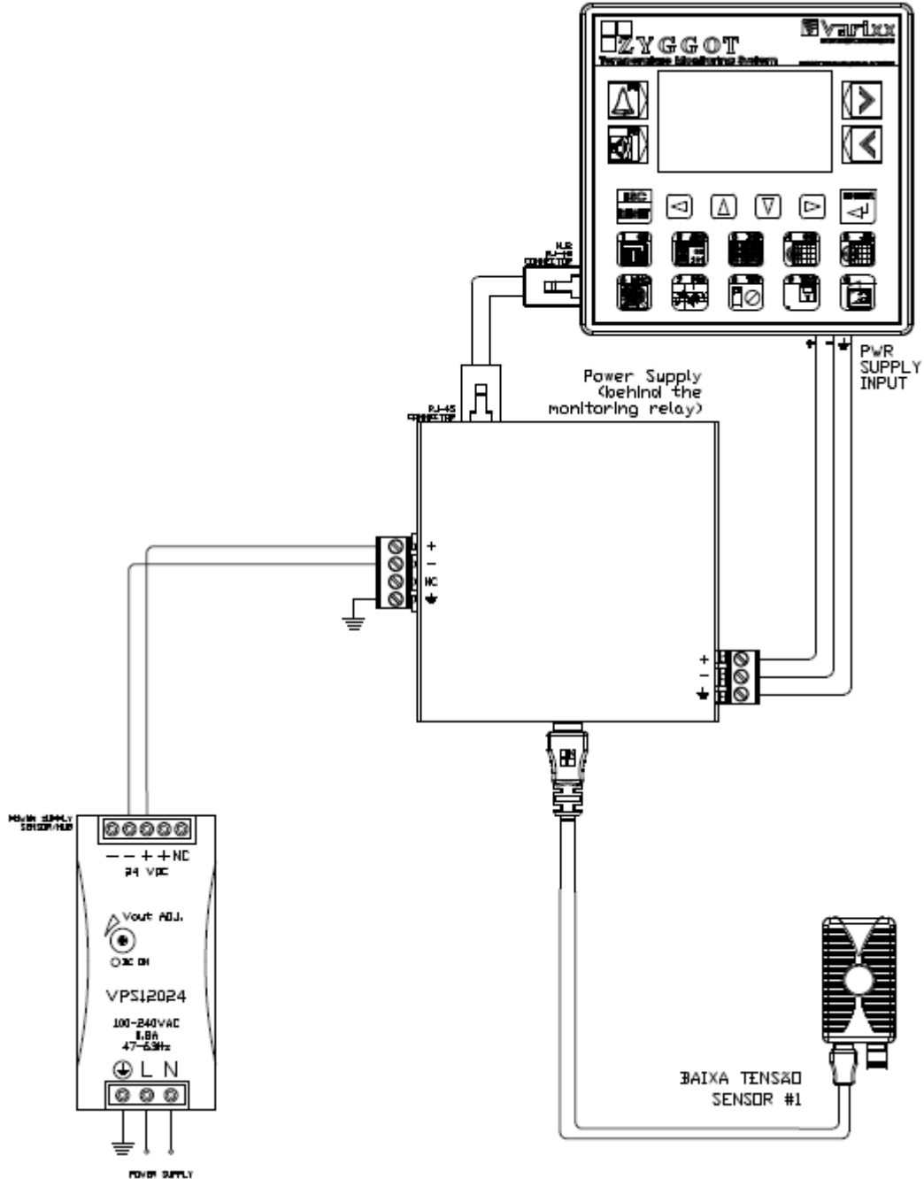
Figure 1 Configuration (default)
