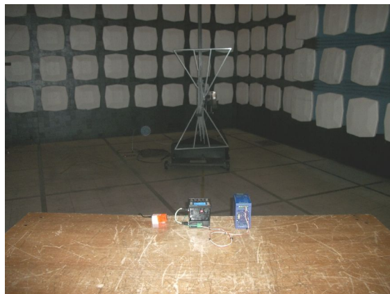
Photos 9 and 10 - Radiated emission
