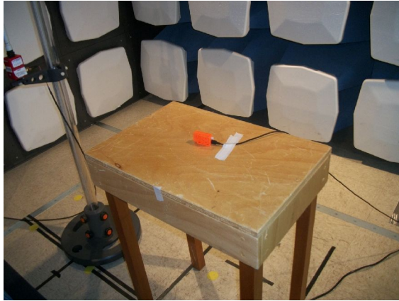
Photos 13 and 14 - Radiated Disturbance Immunity
