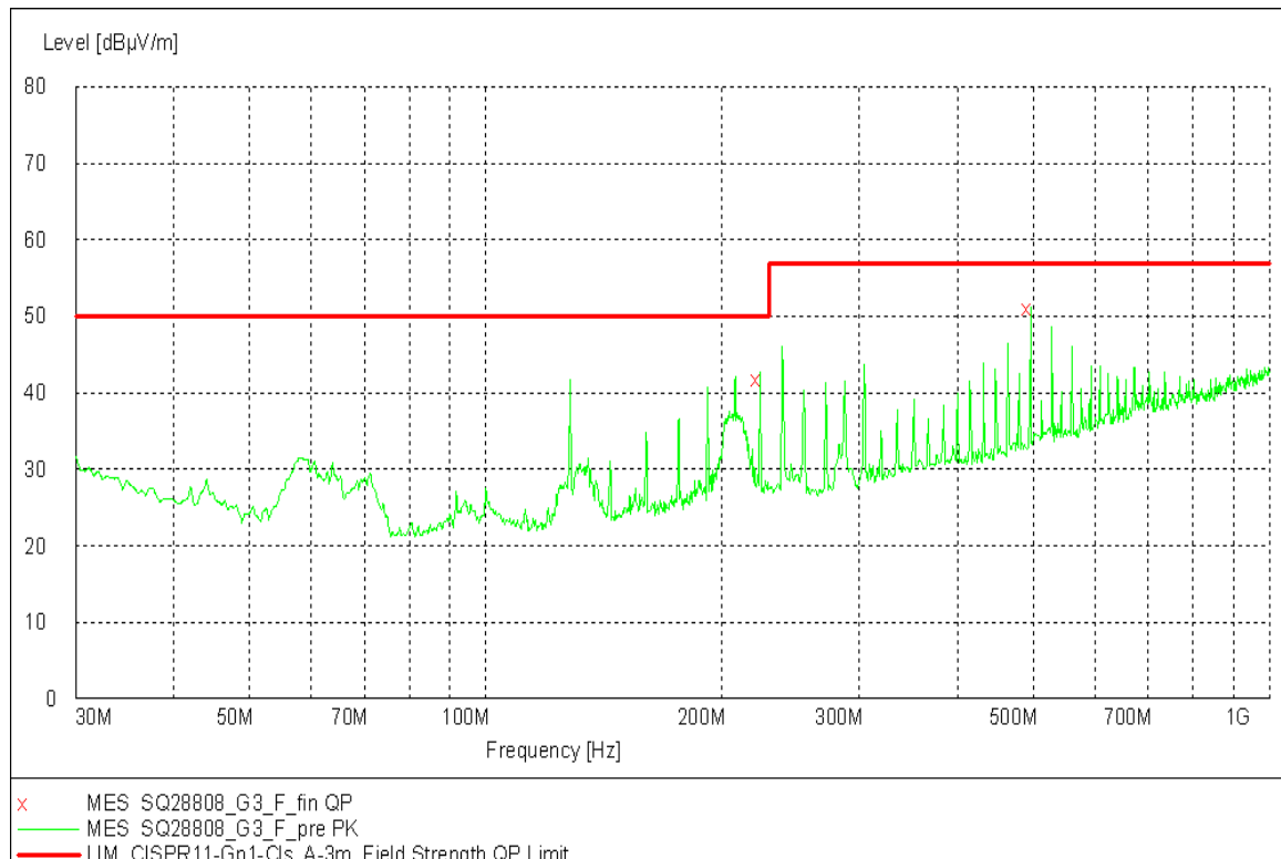
Graph 1 Radiated Emission Test Results – Default Configuration – Power Supply 220V @ 60 Hz (24 Vdc output) – Sample 5252
