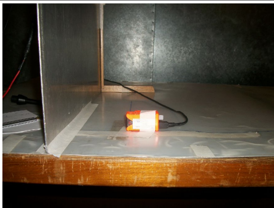
Photo 21 Horizontal rear view and vertical right view of EUT
